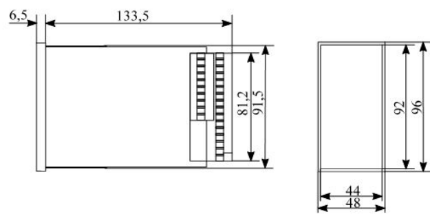
Housing dimensions baelz 6597
