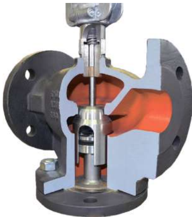
Sectional view of baelz 340-2-B-EMF plug
