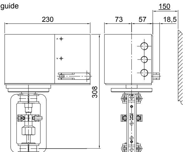
Dimensions of baelz 373-E65 actuator
