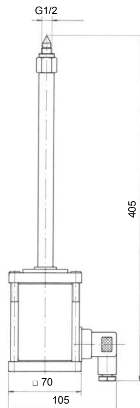
baelz 265st-K 16
