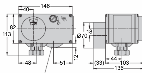
baelz 373-ESA-D-05-35-230
