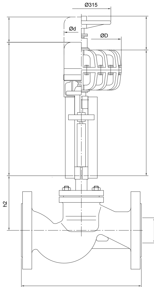
Dimensions baelz 358-K / 359-K, DN 65 - DN 125
