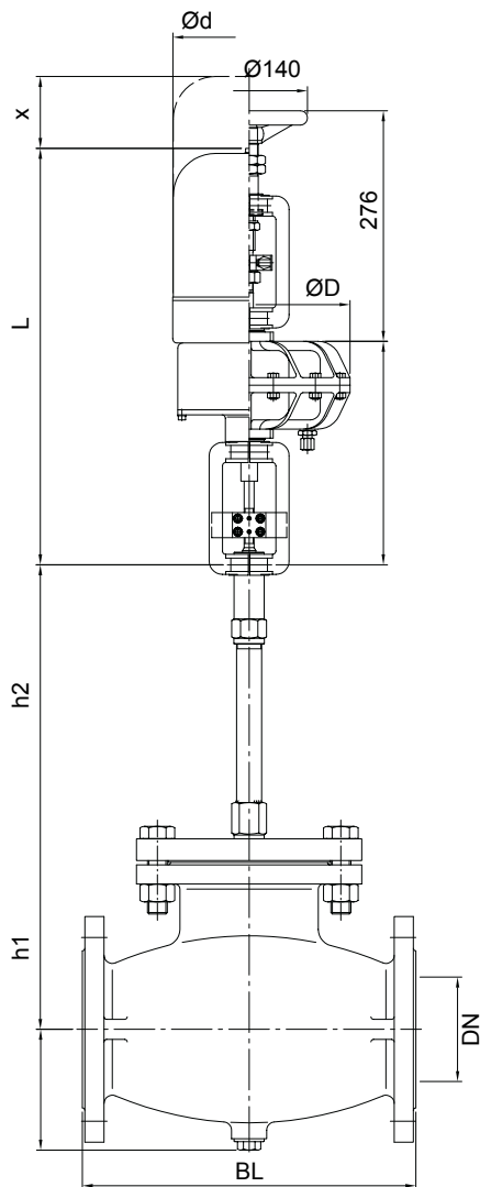
Dimensions 360-EM-C-K 40-125
