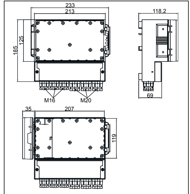
Dimensions 6164B-W2, wall-mounted unit
